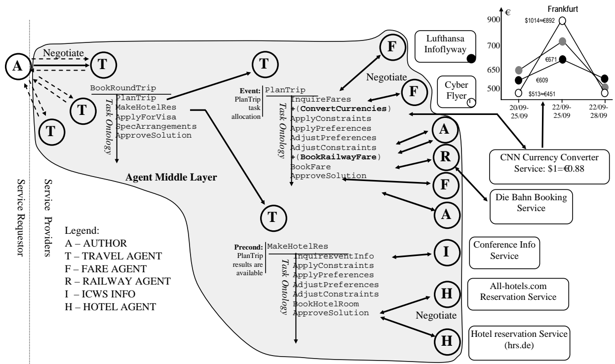
Figure 1: "BookRoundTrip" task execution and service composition
