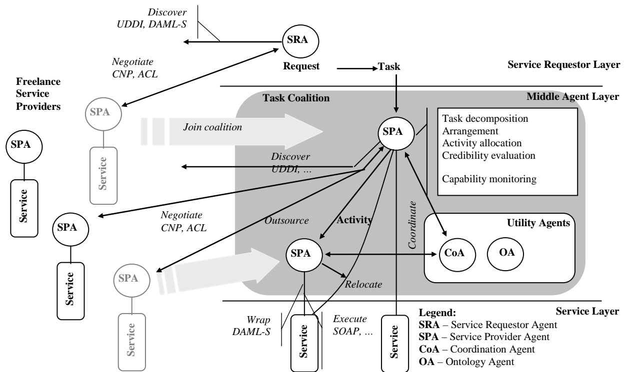
Figure 3: Agent-Based Service Provision Mediation Framework
